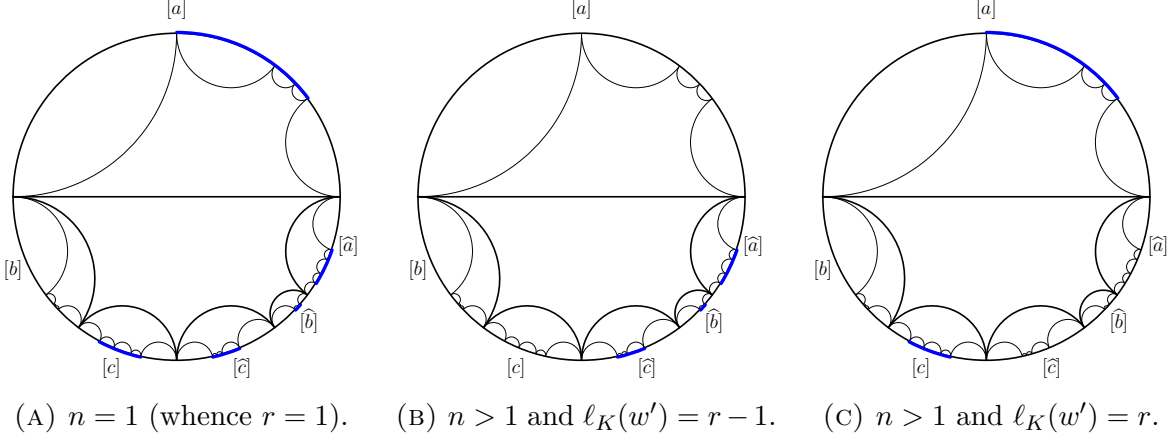
FIGURE 2. Domain D_K(w, r) of h_{w,r} \in \mathcal{H}^r (underlined in blue), when the last letter of w = a_1 \cdots a_n is a_n = \widehat{b} , depending on the value of n and \ell_K(w') , where w' = a_2 \cdots a_n . If r = 1 only cases (A) and (C) appear, since \ell_K(w') = 0 implies n = 1 .
