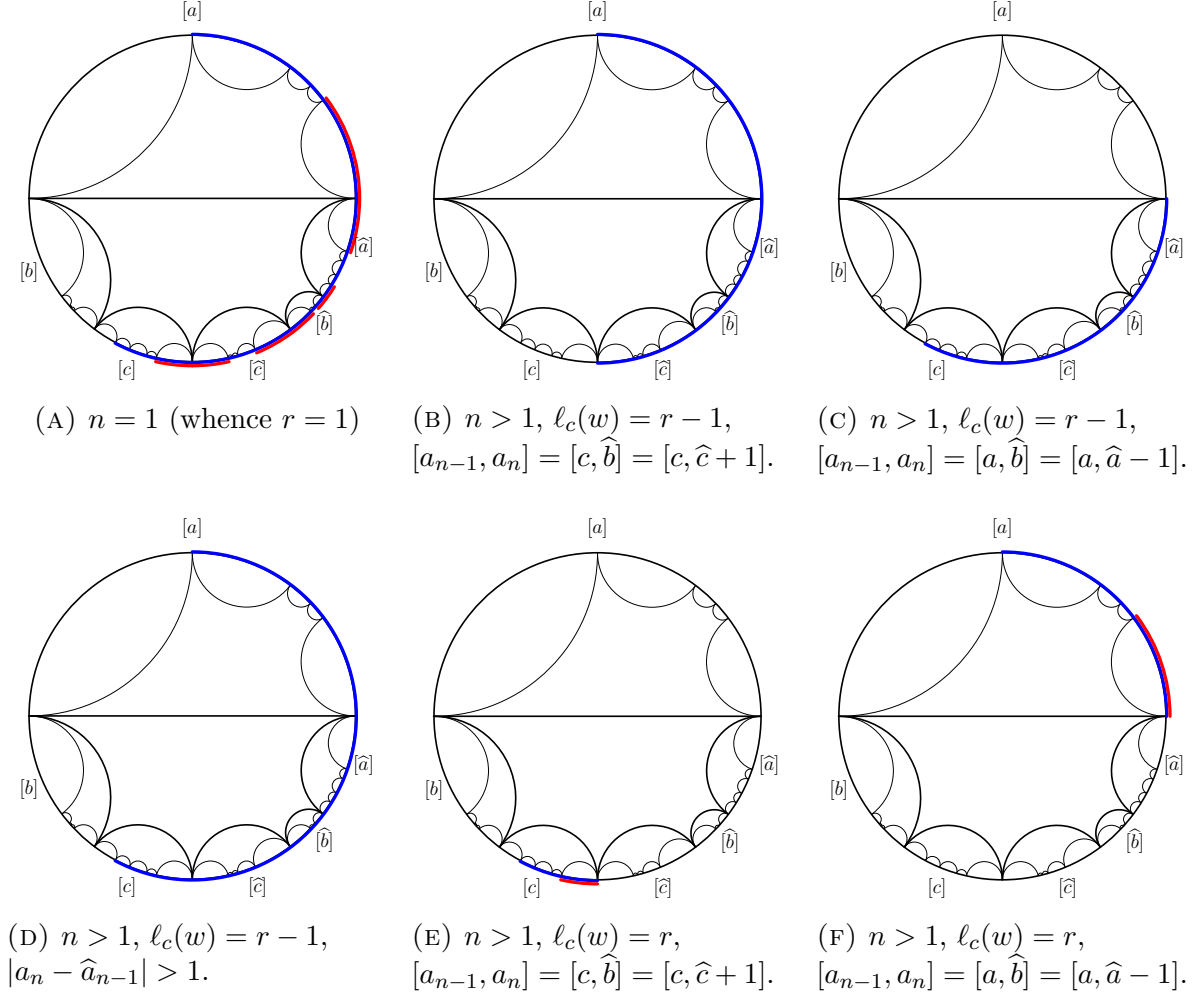
FIGURE 3. Domain D_c(w, r) of h_{w,r}^c \in \mathcal{H}_c^r (underlined in blue), where the last letter of w = a_1 \cdots a_n is a_n = \hat{b} , depending on the value of n and \ell_c(w) and a_{n-1} . If r = 1 only case (A), (E) and (F) appear. The restricted domain D_c^\sharp(w) (for r = 1 ) is highlighted in red.
